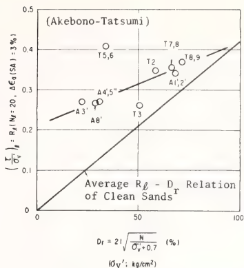
Fig. 26 D_r - R_l Relationship of Sands of Akebono-Tatsumi Site
